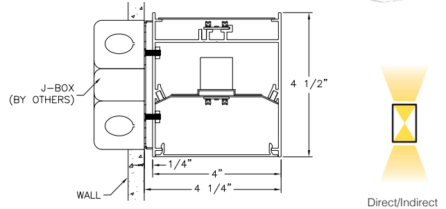
Indirect clear acrylic (CA) lens w/Direct flush lens (FL) shown.
