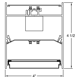
Satin Ice Lens Internal Cross Blade (SIL)
