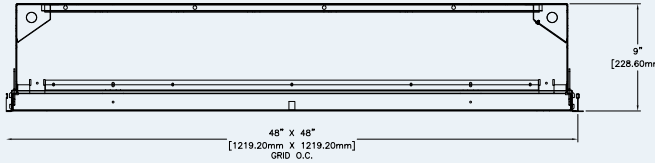
Grid Ceiling Flat Lens. See page 2 for all lens and ceiling options.
