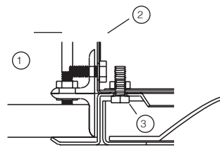
Flange Detail
